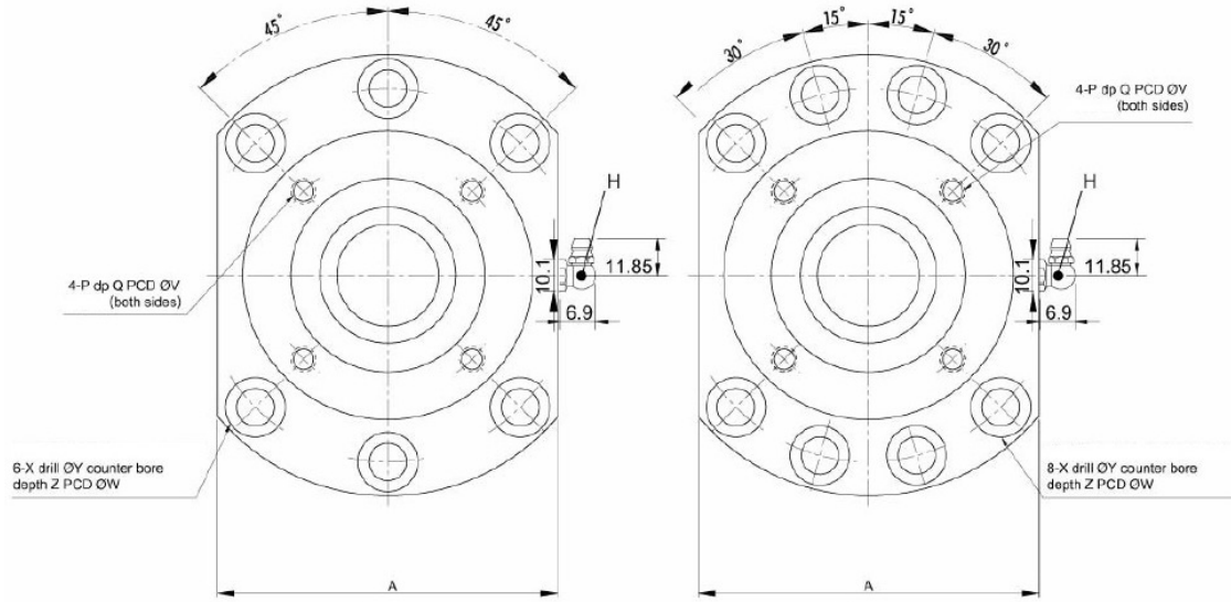
Shaft diameter \varnothing d \leq 30
