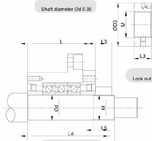
Dimensions of shaft end
